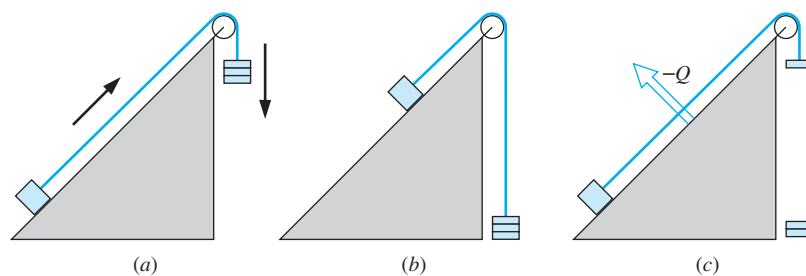
FIGURE 5.14 Demonstration of the fact that friction makes processes irreversible.
