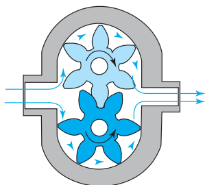
(a) Gear pump
