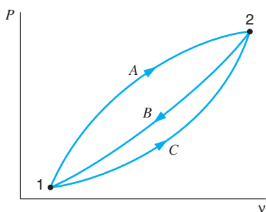
FIGURE 6.4 Two reversible cycles demonstrating that entropy is a property of a substance.
